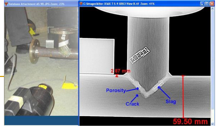
Radiographic testing
